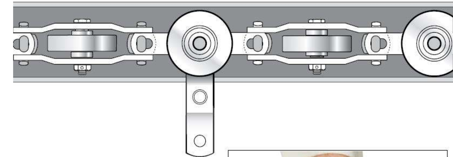
Unibilt® Heavy-Duty Chain With Symmetrical Chain Pin
